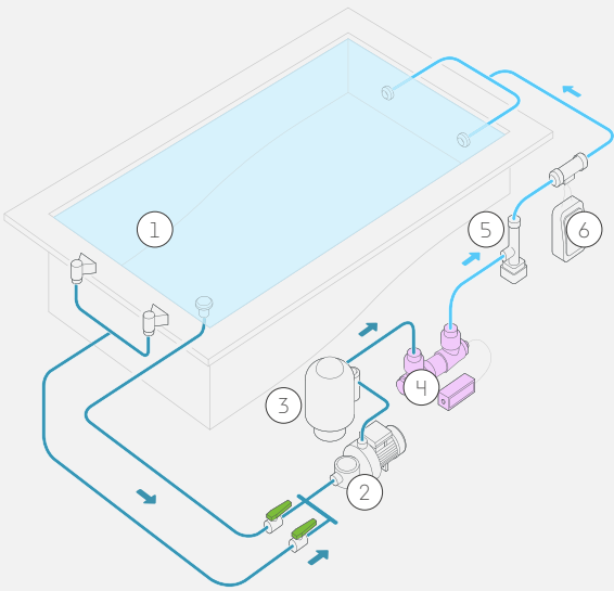
Installation: fresh water and salt water pools
